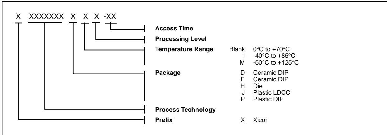
FIGURE 11: XICOR
