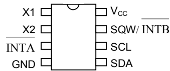
8-Pin DIP (300mil)
