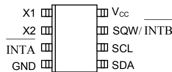
8-Pin SO (150mil)
