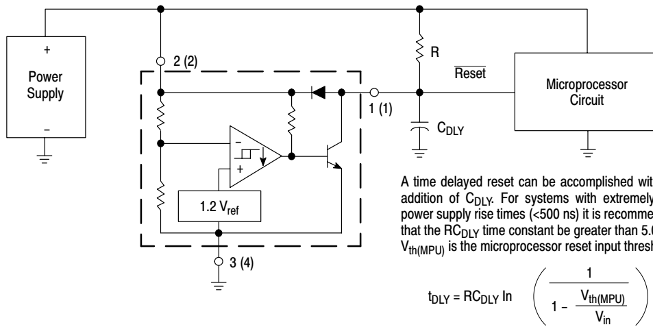
Figure 8. Low Voltage Microprocessor Reset
